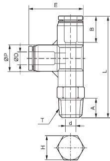
EPD T型分支螺紋三通 Branch Tee
